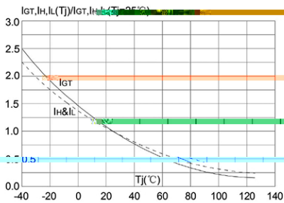
FIG.6: Relative variation of I_{GT} , I_{H\&L} and I_{GT} versus temperature
